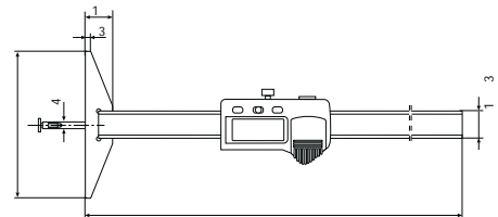
Disc measuring insert
